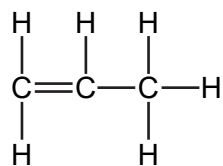
propene
