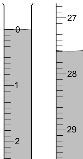
1st titration
