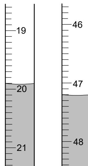
3rd titration
